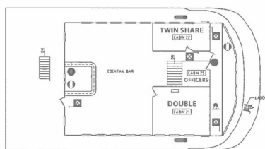
WHEELHOUSE DECK PLAN
